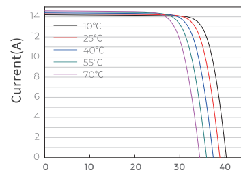
Current-Voltage Curve JAM54D41-440/LB
