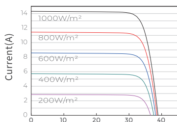
Current-Voltage Curve JAM54D41-440/LB
