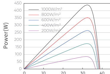
Power-Voltage Curve JAM54D41-440/LB
