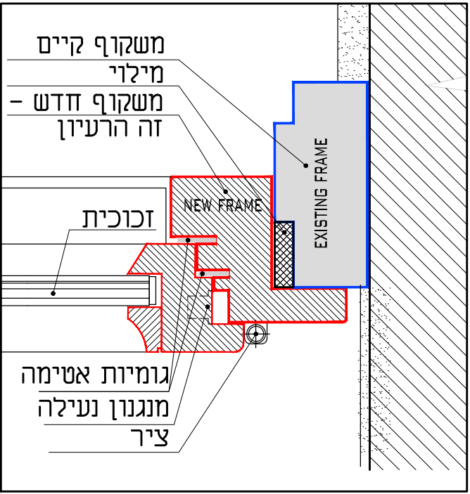
HORIZONTAL SECTION
