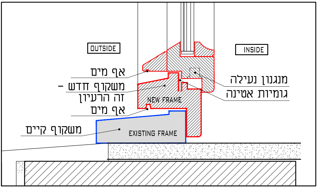
VERTICAL SECTION
