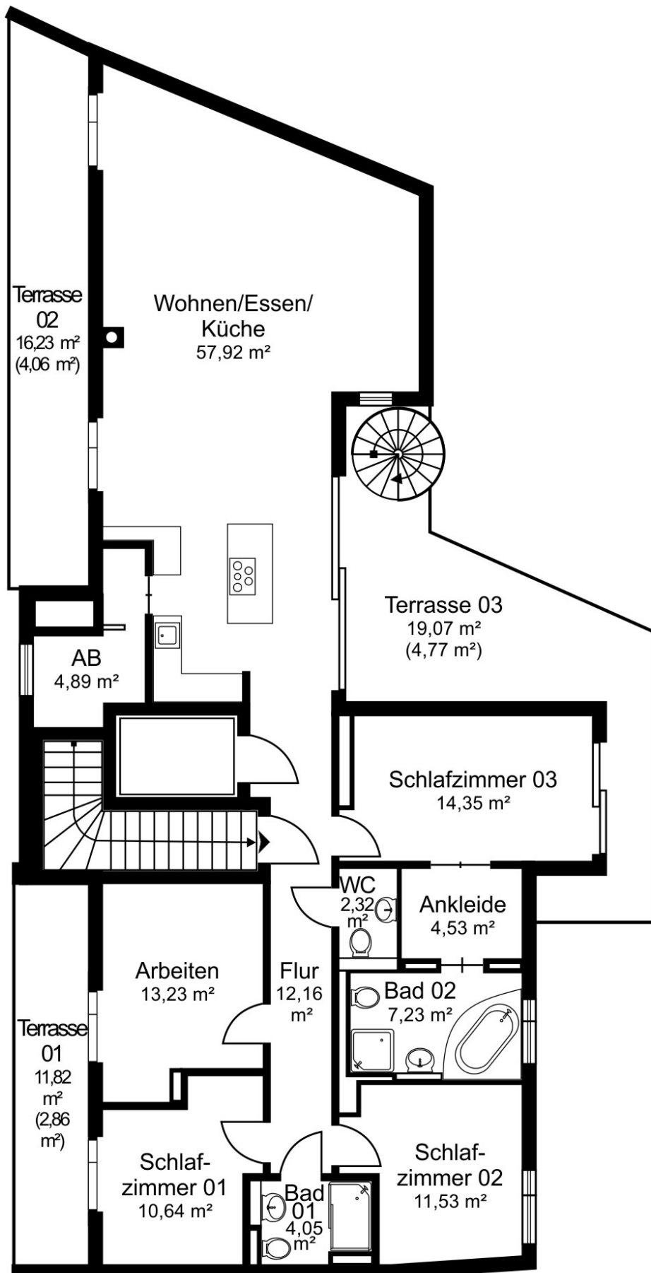
Grundriss Penthouse
