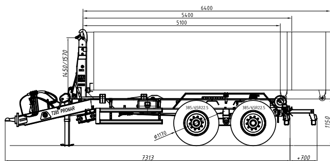
PRONAR T285
