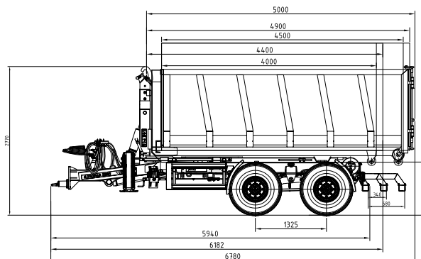
PRONAR T185/1
