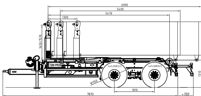
PRONAR T286
