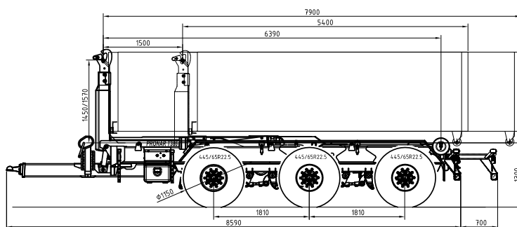
PRONAR T386
